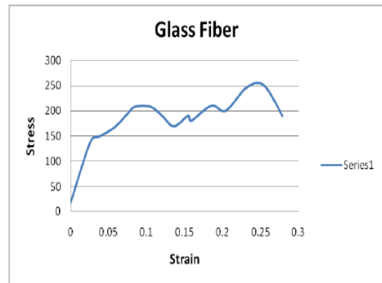
Fig 4(b): Stress-Strain Diagram for Glass Fiber - Specimen-II
